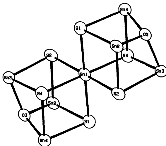
FIGURE 2 ORTEP plot showing the tin-sulfur-oxygen core of the [(n\text{-BuSn}(\text{S})\text{O}_2\text{PPh}_2)_3\text{O}]_2\text{Sn} molecule. Atoms with the same label are related by a crystallographic inversion center ( -x, -y, -z ).
