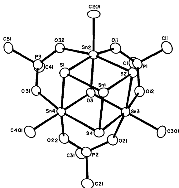
FIGURE 1 ORTEP plot of the asymmetric unit of the [(n\text{-BuSn}(\text{S})\text{O}_2\text{PPh}_2)_3\text{O}]_2\text{Sn} molecule with thermal ellipsoids at the 30% probability level. Atom Sn1 lies on a crystallographic inversion center. Pendant carbon atoms of the six phenyl groups and of the three n -butyl groups are omitted for purposes of clarity. Average bond lengths ( \text{\AA} ): Sn1—S = 2.561 (1); Sn—S = 2.576 (1); Sn—C = 2.151 (6); Sn—O3 = 2.100 (4); Sn—O = 2.147 (4); P—O = 1.515 (4). Average bond angles (deg): S—Sn1—S = 90 (av value required by symmetry), 180 (required by symmetry); S—Sn—S = 89.41 (4); S—Sn—O3 = 82.2 (1); S—Sn—O = 90.9 (1), 167.1 (1); S—Sn—C = 101.9 (2); O—Sn—O3 = 85.1 (1); O—Sn—O = 86.0 (1); C—Sn—O3 = 174.1 (2); C—Sn—O = 96.3 (2); Sn—O3—Sn = 109.4 (1); Sn—O—P = 132.5 (2); Sn1—S—Sn = 90.18 (4); Sn—S—Sn = 83.38 (4). Sn refers to Sn2—Sn4. O refers to phosphinate oxygen atoms. The unique O3 and Sn1 are so designated.
